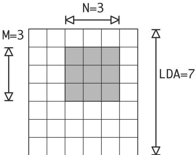
Figure 6.4: Memory layout of a row and column of a matrix in column-major storage
