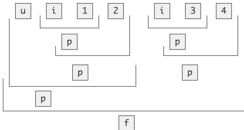
Figure 20.1: Reduction of four items on two threads, taking into account initial values.
