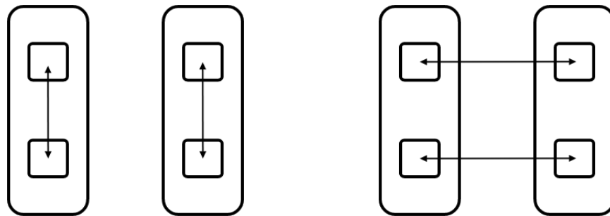
Figure 16.1: Intra and inter schemes for bandwidth
