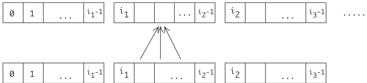
Figure 4.1: Three point averaging in parallel, case of interior points
